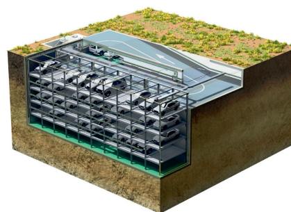
Combiparker 560
