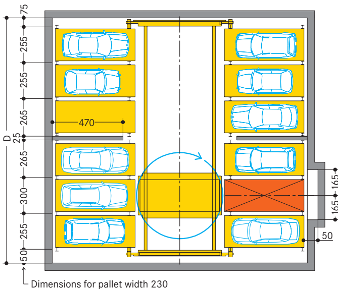
Dimensions in cm
